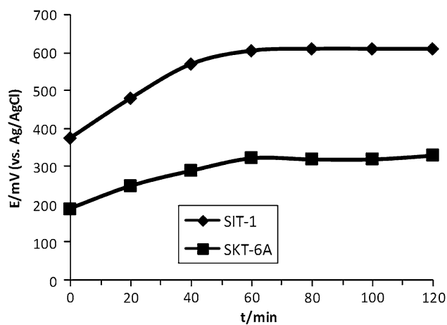
Fig. 2 Open circuit potentials of SIT-1 and SKT-6A versus time for Medinal adsorption
