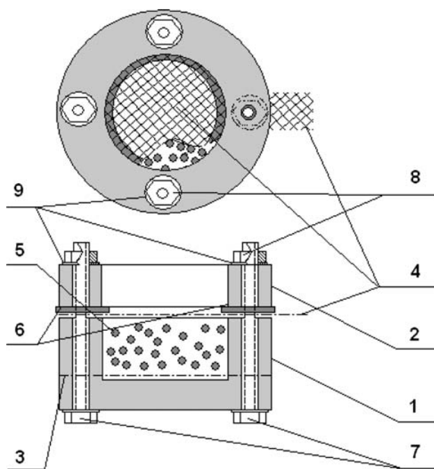
Fig. 1 Column for granulated carbon potential measurements
